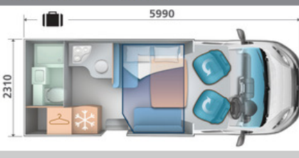
T-LINE 590 LAYOUT
